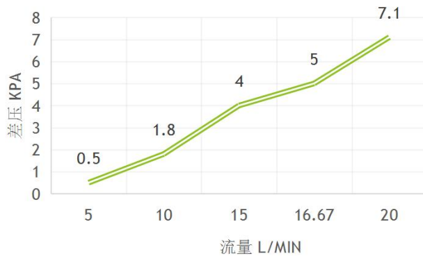
CHEP-02采暖压差曲线
